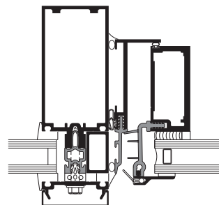
JAMBA
